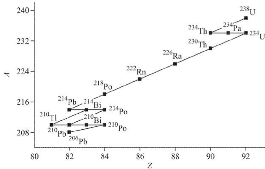
Figure 3.5 A = 4n + 2 , Uranium series. End product is ^{206}\text{Pb} .
