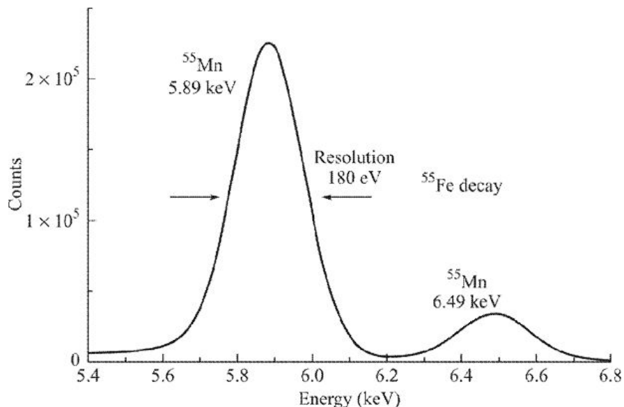
Figure 7.16 X-ray spectrum of ^{55}\text{Fe} as recorded by Si(Li) detector.
