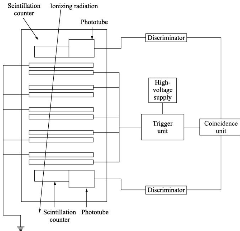
Figure 7.21 Spark chamber.
