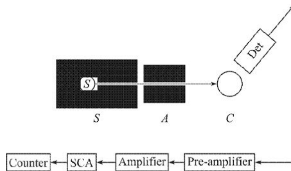
Figure 5.9 Experimental set-up to verify Compton effect.
