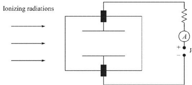
Figure 7.4 Ionization chamber.
