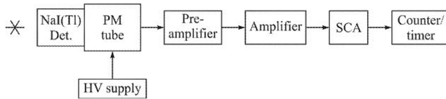
Figure 7.10 Block diagram of a scintillation spectrometer.
