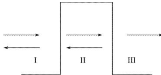
Figure 3.18 The rectangular potential barrier V(x) versus x .
