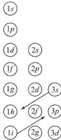
Figure 2.3 Way to remember the square well potential levels.
