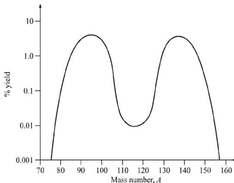
Figure 4.4 Per cent yield of different fission fragments in fission of ^{235}\text{U} .
