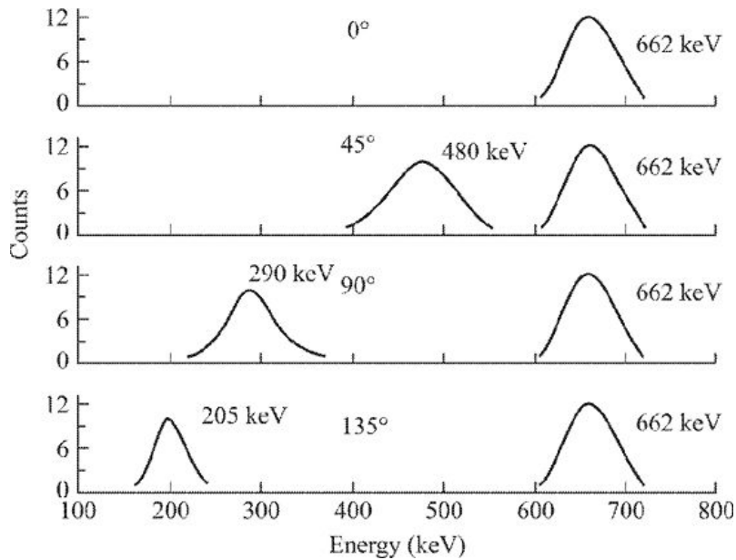
Figure 5.10 Compton scattered 662 keV \gamma -rays of ^{137}\text{Cs} at different angles.
