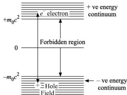
Figure 5.11 Dirac diagram for electron hole (positron) production.
