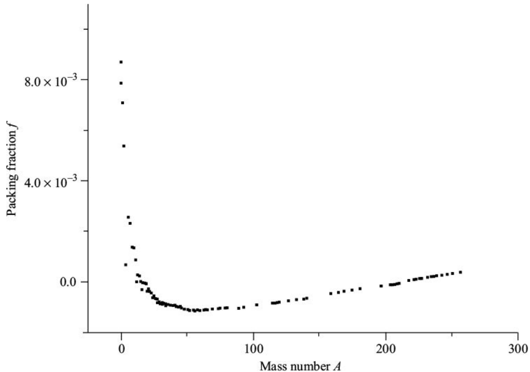
Figure 1.3 Packing fraction f versus mass number A .
