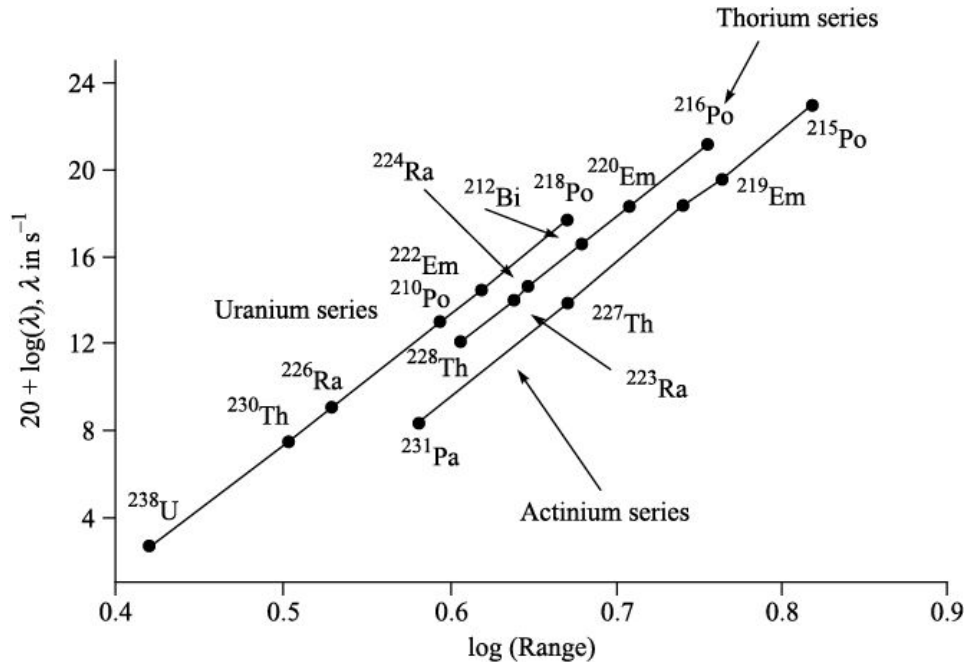
Figure 3.16 Plot of \log(\lambda) versus \log(\text{Range}) for uranium, thorium and actinium series.
