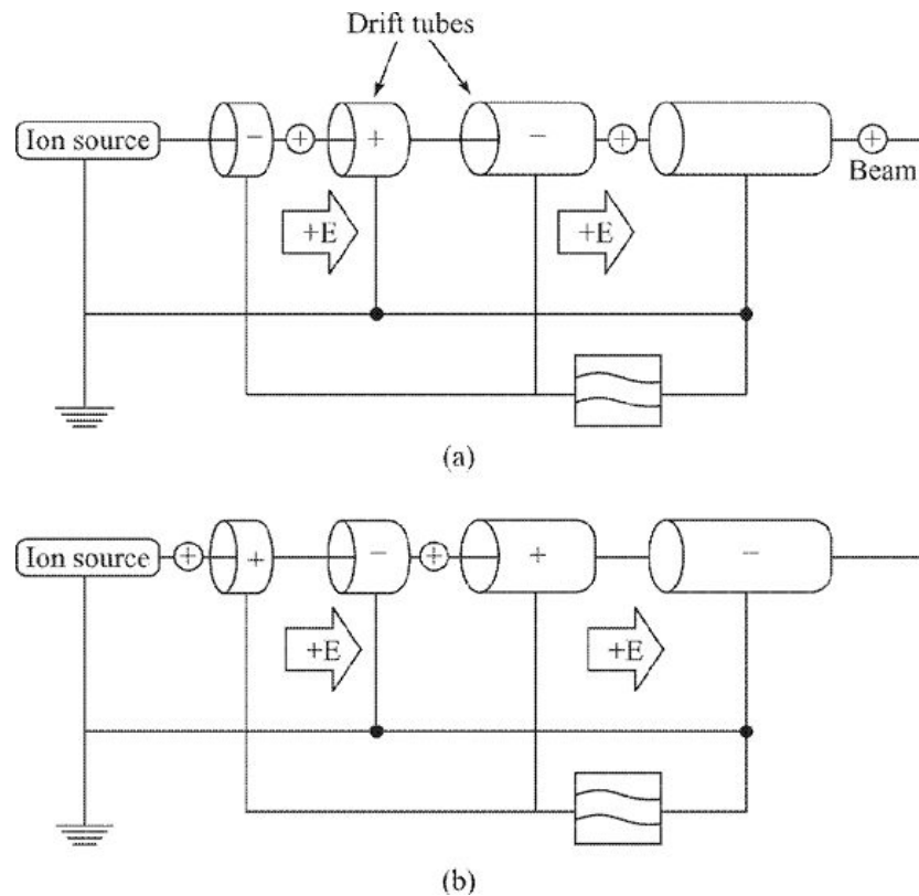
Figure 6.4 (a) the first drift tube is negatively charged. It means beam of +ve ions will be accelerated, (b) the first drift tube is positively charged. It means beam of +ve ions will not be accelerated.
