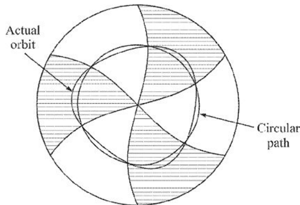
Figure 6.12 High-field and low-field regions in an A.V.F. cyclotron. Particles perform radial oscillations about the circular path.
