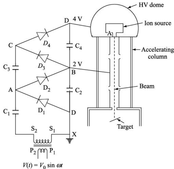
Figure 6.1 Cockcroft and Walton accelerator.
