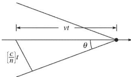
Figure 7.22 Cerenkov radiations wavefront in a medium.
