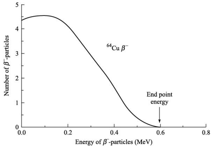
Figure 3.19 Spectrum of \beta^- -particles emitted in the decay of ^{64}\text{Cu} .
