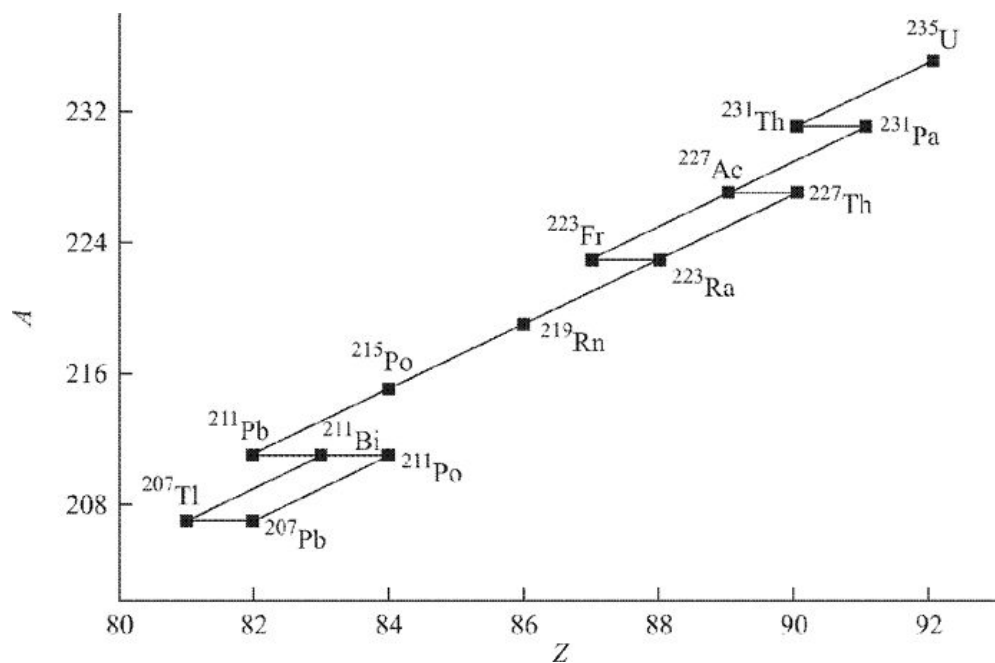
Figure 3.6 A = 4n + 3 , Actinium series. End product is ^{207}\text{Pb} .
