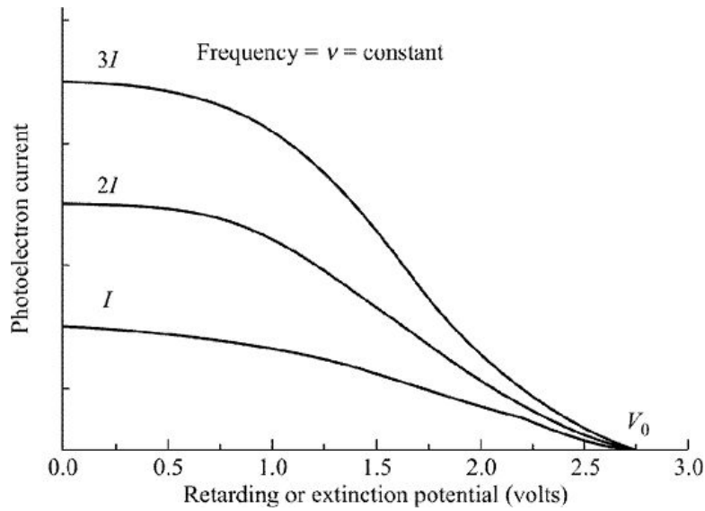
Figure 5.6 Photoelectric current versus retarding potential for various intensities of incident light.
