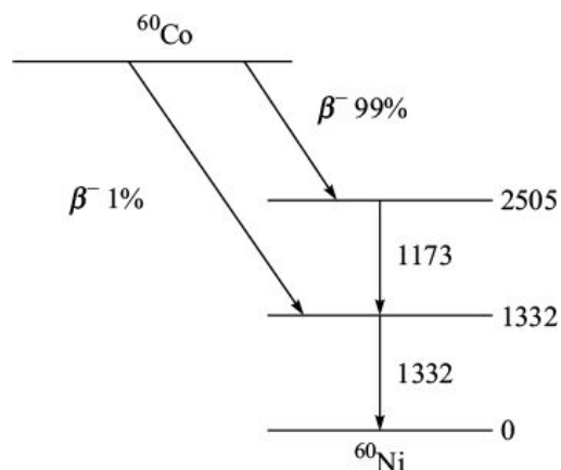
Figure 3.24 Decay scheme of ^{60}\text{Co} .
