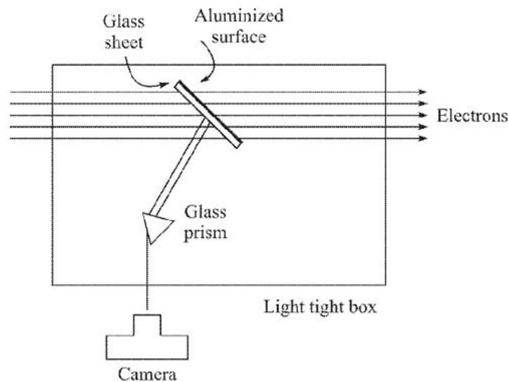
Figure 7.23 Cerenkov detector.
