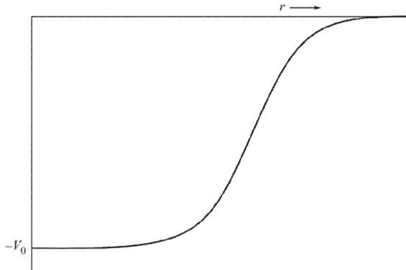
Figure 2.8 Wood–Saxon potential.
