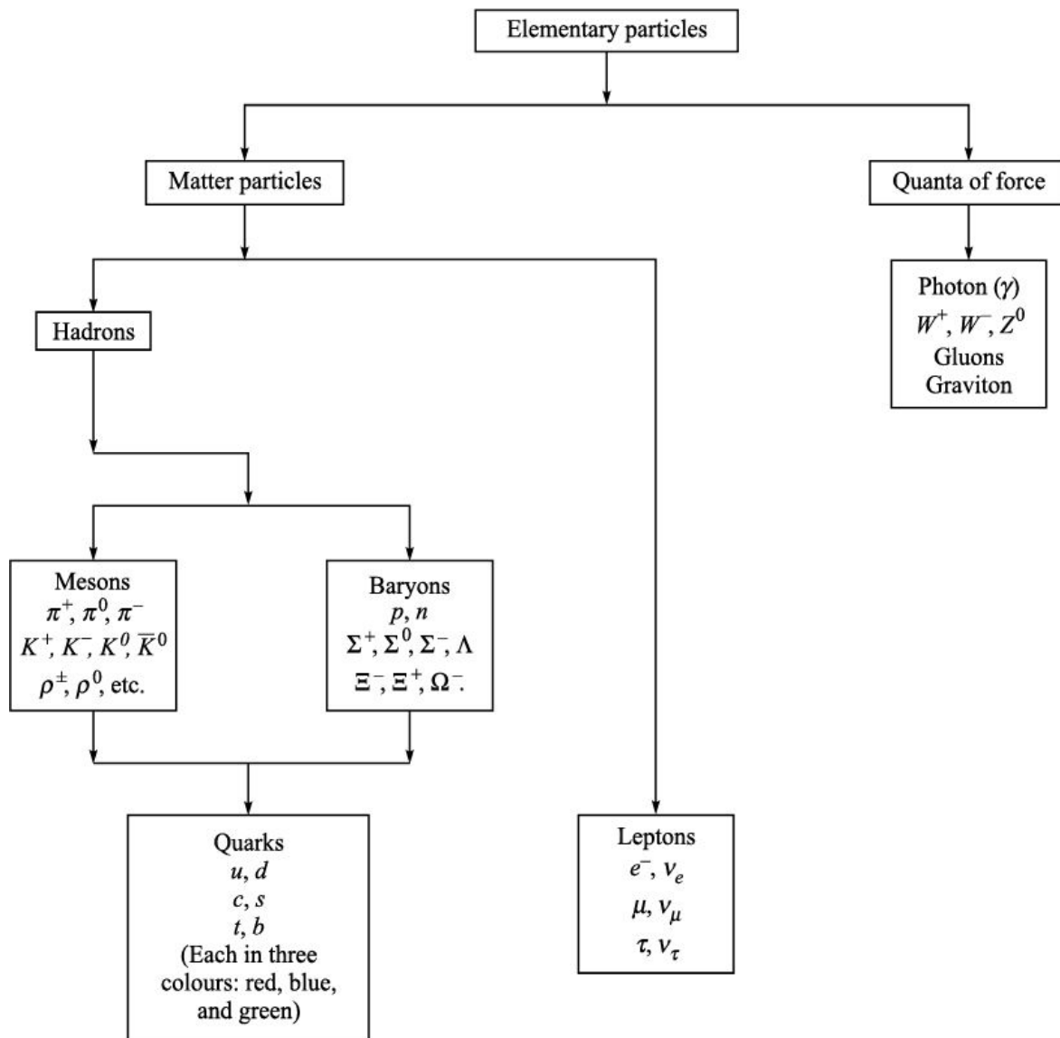
Figure 8.1 Classification of elementary particles.
