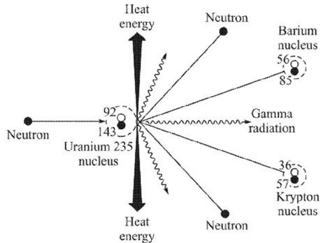
Figure 4.3 Schematic diagram of fission of ^{235}\text{U} by neutrons.
