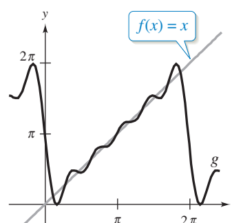
Fifth-Order Fourier Approximation
