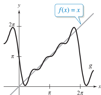
Fourth-Order Fourier Approximation
