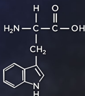
Tryptophan (Trp, W)
