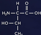
Threonine (Thr, T)
