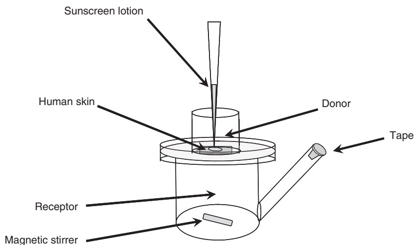
Figure 9.1.6 The Franz's diffusion cell consists of an upper donor and a lower receptor chamber, separated by a skin preparation. The test substances (e.g. sunscreen lotion) that are applied on the stratum corneum faces the donor compartment. The receptor fluid is well mixed (magnetic stirrer) throughout the experiment (adapted from Balaguer et al. , 2006).
