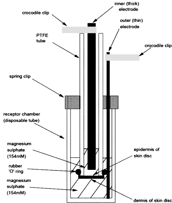
Figure 9.1.1 Device to determine the transcutaneous electrical resistance (TER) test through the rat skin disc (B.40. Skin corrosion, Directive 2000/33/EC).
