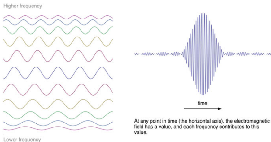
Fig. 10.5 A localised wave packet as a superposition of plane waves. The interactive figure is available online (see supplementary material 5)
