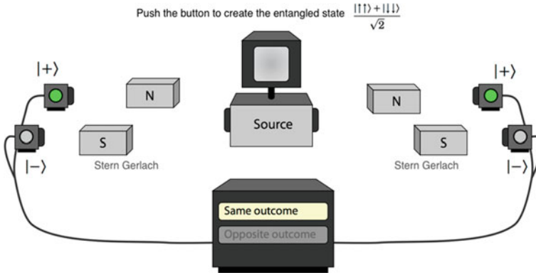
Fig. 6.3 Creating quantum correlations. The interactive figure is available online (see supplementary material 3)
