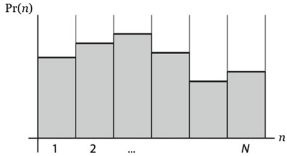
Fig. 8.1 Discrete position probabilities
