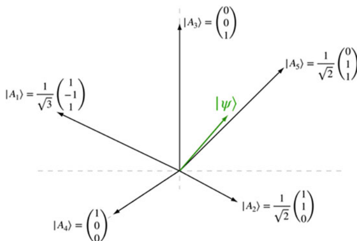
Fig. 10.4 Contextuality in three dimensions. The interactive figure is available online (see supplementary material 4)
