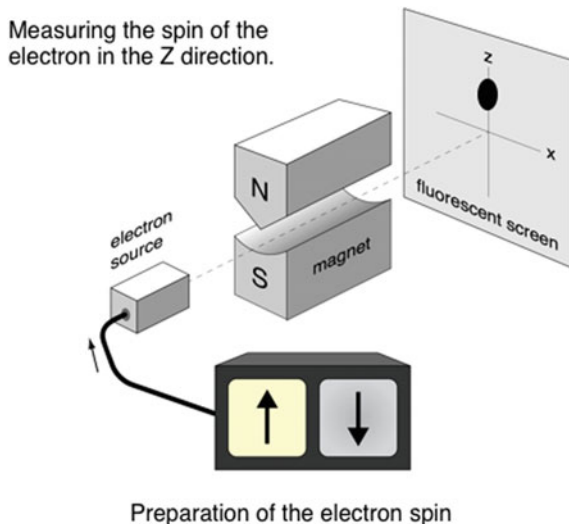
Fig. 3.1 A Stern–Gerlach apparatus. The “up” and “down” regions on the screen where the electron is detected define the electron spin states |\uparrow\rangle and |\downarrow\rangle . The interactive figure is available online (see supplementary material 1)
