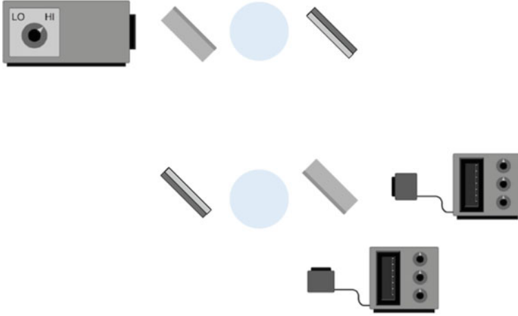
Fig. 7.2 A Mach–Zehnder interferometer where the photon interacts with the environment. The interactive figure is available online (see supplementary material 2)
