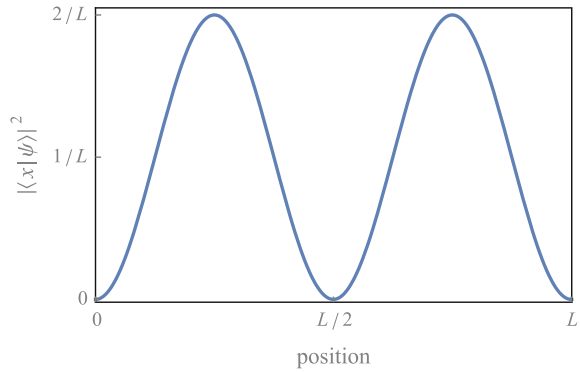
Fig. 8.3 The probability density |\langle x|\psi\rangle|^2 for the position of a particle in a box in the state \psi(x) of Eq. (8.33)
