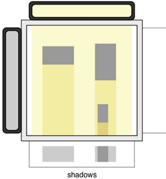
Fig. 3.7 The principle of tomography. The interactive figure is available online (see supplementary material 6)
