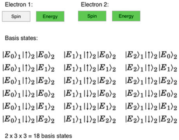
Fig. 6.1 Constructing states for composite systems. The interactive figure is available online (see supplementary material 1)
