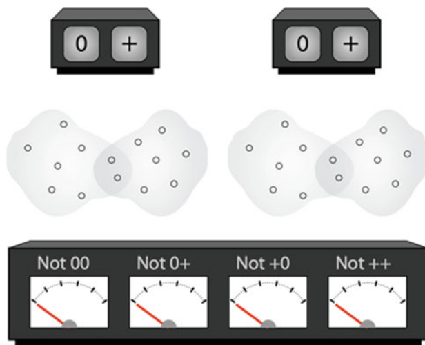
Fig. 10.3 The PBR theorem. The interactive figure is available online (see supplementary material 3)
