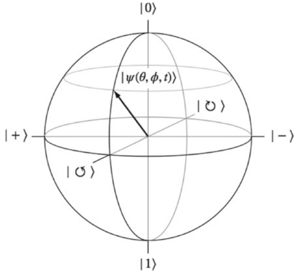
Fig. 4.4 Time evolution as a rotation of the state vector in the Bloch sphere. The interactive figure is available online (see supplementary material 3)
