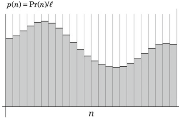
Fig. 8.2 Towards a continuum of probability densities. The interactive figure is available online (see supplementary material 1)
