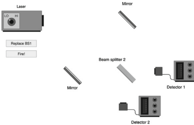
Fig. 7.1 A Mach–Zehnder interferometer with a removable beam splitter. The interactive figure is available online (see supplementary material 1)
