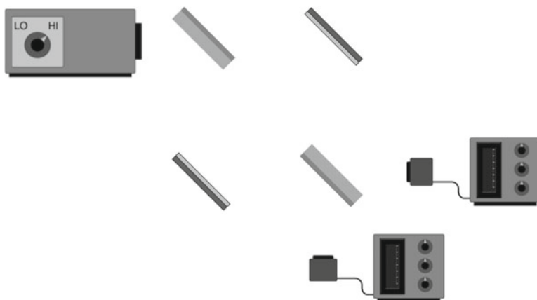
Fig. 1.4 A Mach-Zehnder interferometer. The interactive figure is available online (see supplementary material 4)
