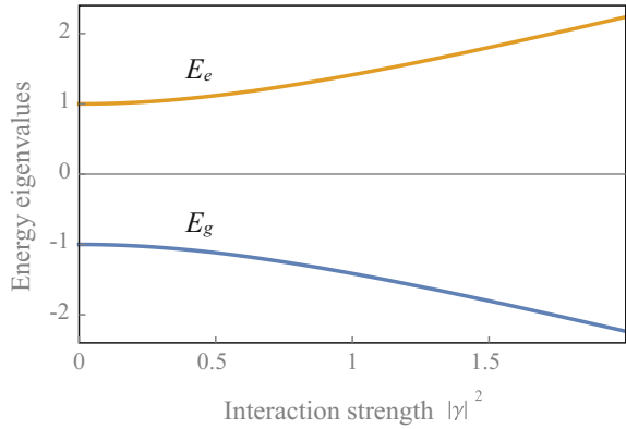
Fig. 5.1 Changes in eigenvalues with increasing interaction strength |\gamma|^2 . The energy units on the axes are arbitrary
