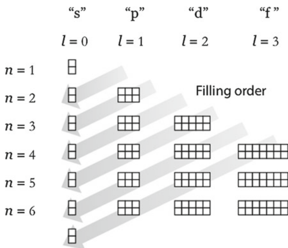
Fig. 8.11 Atom energy shell filling order
