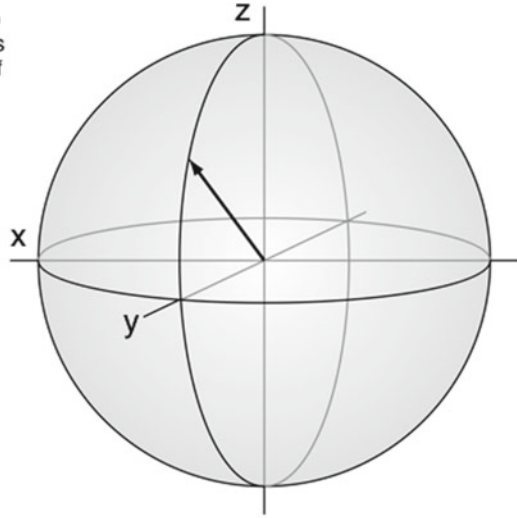
Fig. 3.5 Projections in the Bloch sphere. The interactive figure is available online (see supplementary material 4)
