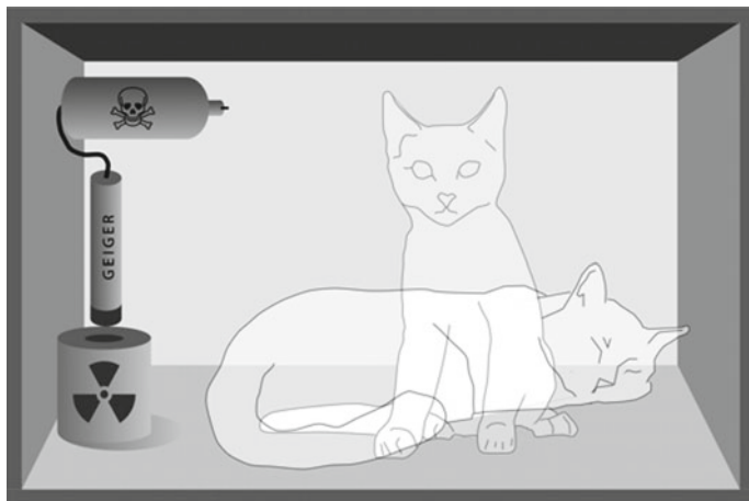
Fig. 10.1 Schrödinger's cat. The interactive figure is available online (see supplementary material 1)
