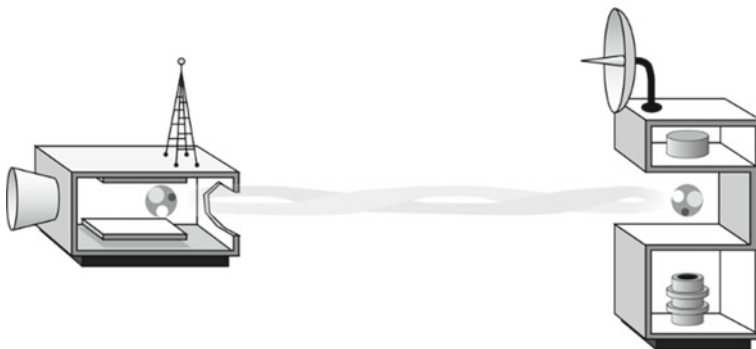
Fig. 6.5 Inside the teleportation machine. The interactive figure is available online (see supplementary material 5)
