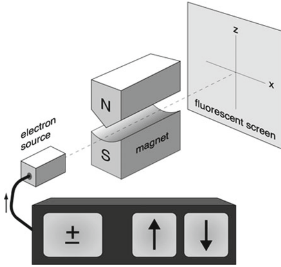
Fig. 3.2 Creating electrons in spin states |\pm\rangle will give different probabilities of finding the electron in the “up” and “down” regions. The interactive figure is available online (see supplementary material 2)
