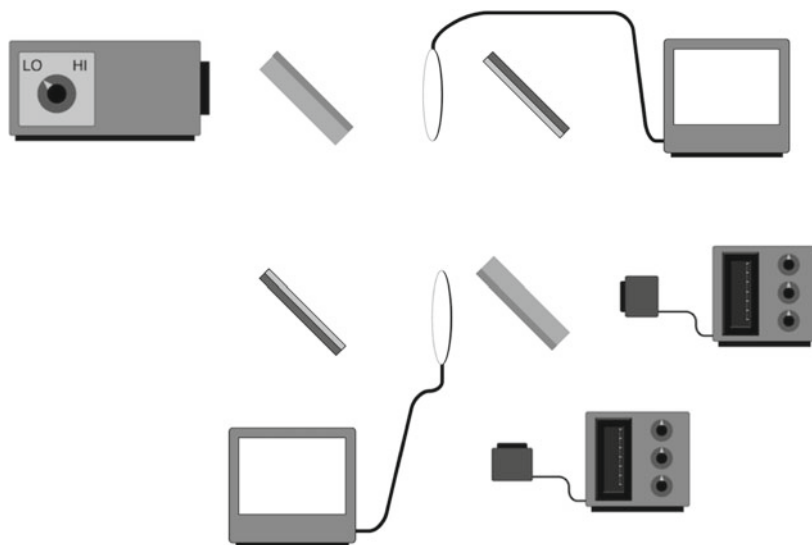
Fig. 1.6 A Mach–Zehnder interferometer with QND measurements of the photon path. The interactive figure is available online (see supplementary material 5)
