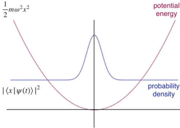
Fig. 9.5 The coherent state for the pendulum. The interactive figure is available online (see supplementary material 4)
