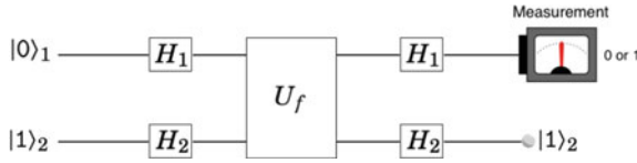
Fig. 6.6 Deutsch' algorithm in circuit form, with the Hadamard operators H_1 and H_2 , and the single function call U_f . The interactive figure is available online (see supplementary material 6)
