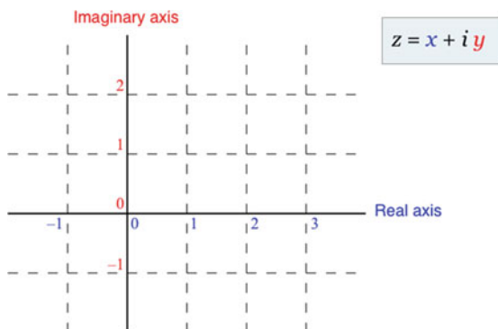
Fig. 2.5 The plane of complex numbers. The interactive figure is available online (see supplementary material 3)
