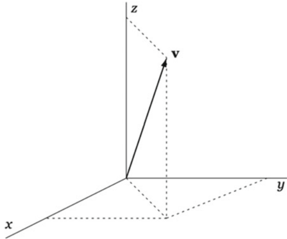
Fig. 5.2 Projections of vectors. The interactive figure is available online (see supplementary material 1)
