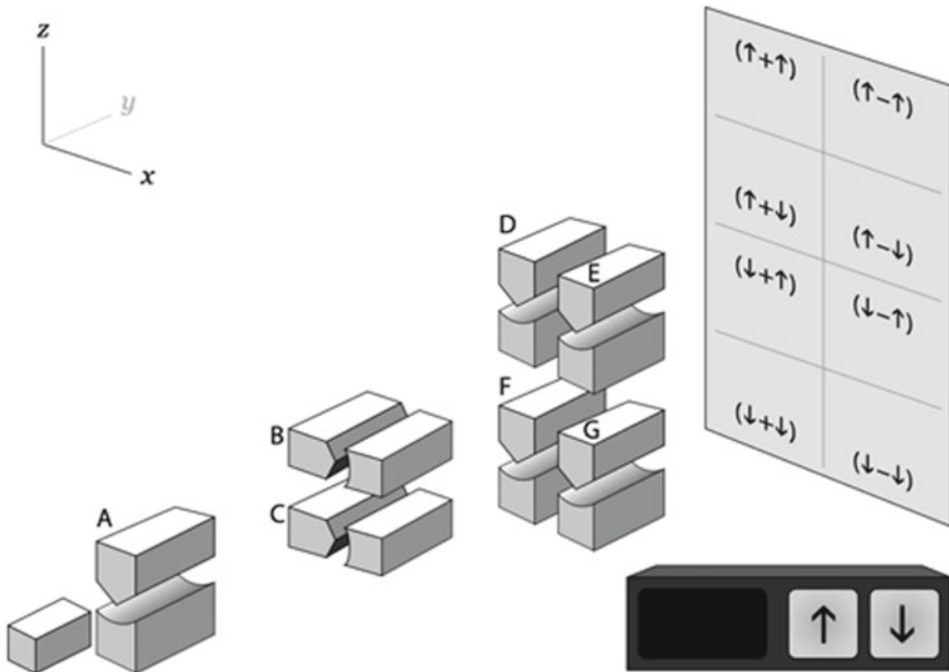
Fig. 9.2 Daisy-chaining three Stern–Gerlach experiments. The interactive figure is available online (see supplementary material 2)
