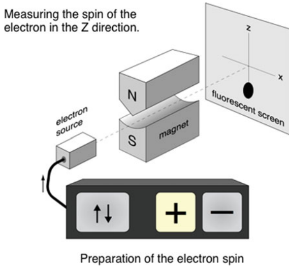
Fig. 3.3 A Stern–Gerlach apparatus with input states |\pm\rangle . The interactive figure is available online (see supplementary material 3)
