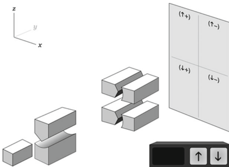
Fig. 9.1 Daisy-chaining two Stern–Gerlach experiments. The interactive figure is available online (see supplementary material 1)
