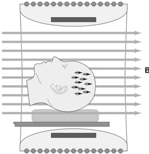
Fig. 3.6 Spins aligned to a magnetic field for magnetic resonance imaging. The interactive figure is available online (see supplementary material 5)
