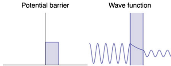
Fig. 8.8 The effect of the barrier on quantum tunnelling. The interactive figure is available online (see supplementary material 4)
