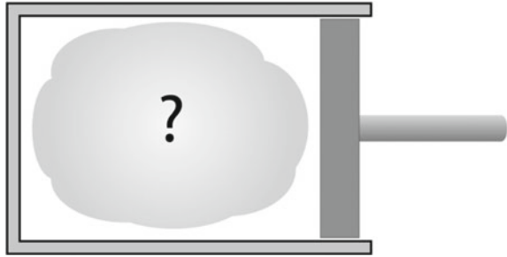
Fig. 7.3 Locating a particle in a box. The interactive figure is available online (see supplementary material 3)
