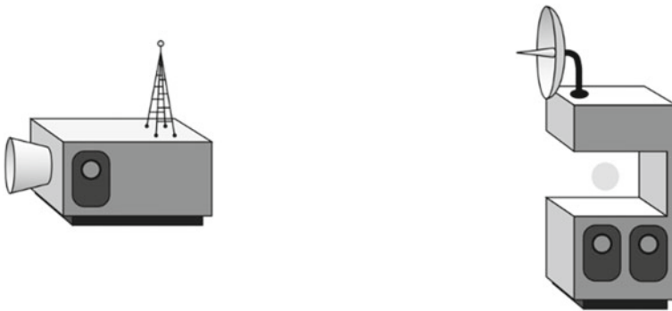
Fig. 6.4 Cartoon of a teleportation machine. The interactive figure is available online (see supplementary material 4)
