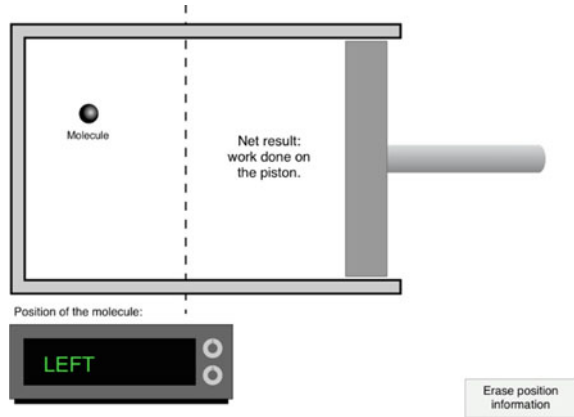
Fig. 7.4 Erasing information will increase the entropy. The interactive figure is available online (see supplementary material 4)
