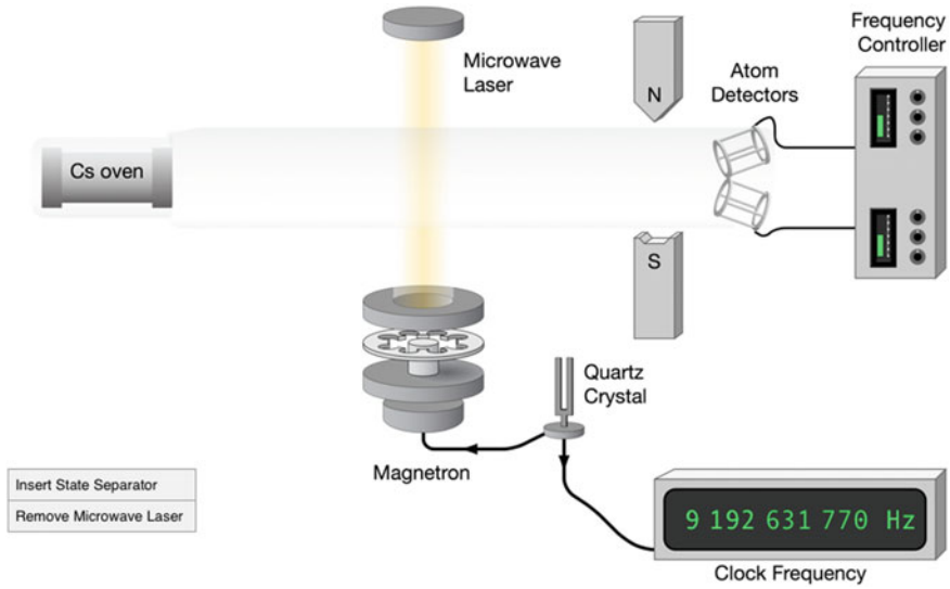
Fig. 4.5 Working principle of the atomic clock. The interactive figure is available online (see supplementary material 4)
