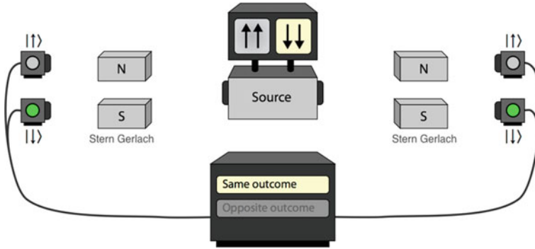
Fig. 6.2 Creating classical correlations. The interactive figure is available online (see supplementary material 2)
