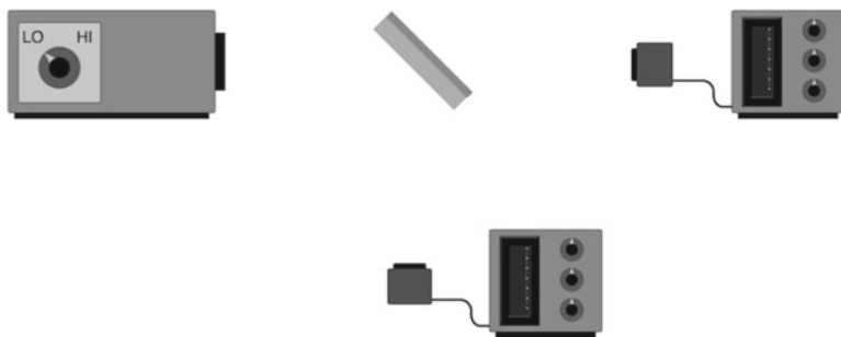
Fig. 1.3 A laser and a beam splitter. The interactive figure is available online (see supplementary material 3)
