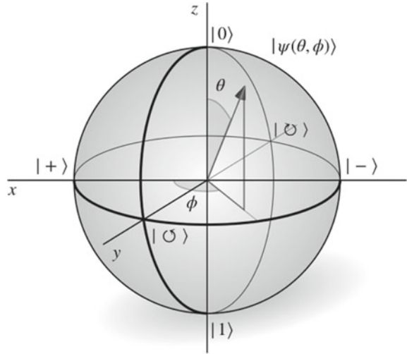
Fig. 3.4 The Bloch sphere
