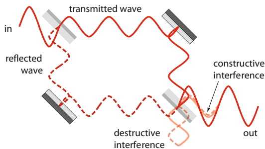
Fig. 1.5 Classical waves in a Mach–Zehnder interferometer. Waves appearing from the second beam splitter with opposite phase cause destructive interference, resulting in a complete absence of light in that output beam. All the light appears in the output with the constructive interference. The amplitude of the wave is the square root of the intensity
