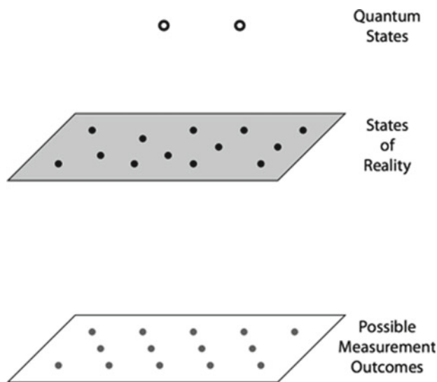
Fig. 10.2 A model of an underlying reality for quantum probabilities. The interactive figure is available online (see supplementary material 2)
